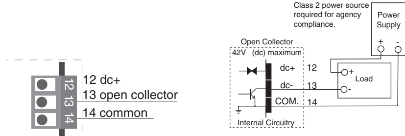
Figure 16b — Output 3 Process
