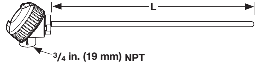
Type 4 - Connection Head Only with 1/2 inch NPT process connection
