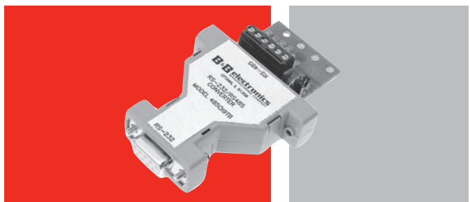
0830-0473-0005 232 to 485, Isolated, DB9 Female to Screw Terminals
