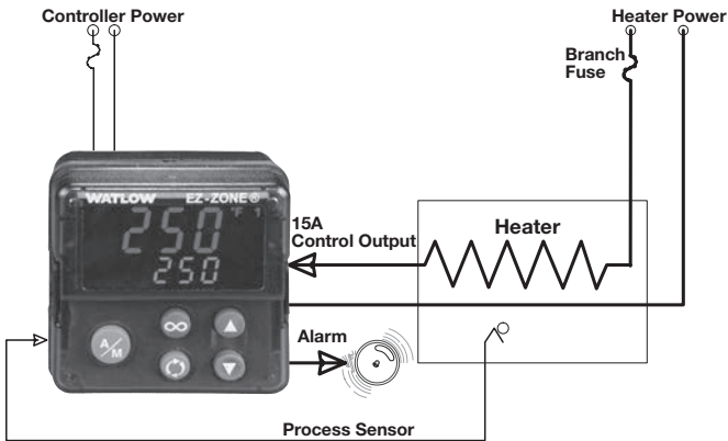
EZ-ZONE PM EXPRESS PID Model
